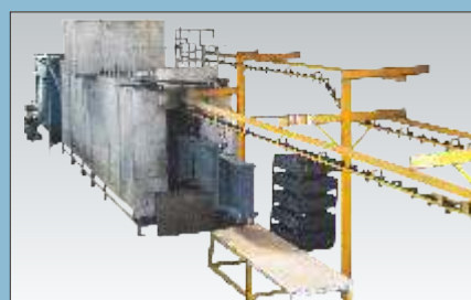
Powder Coating Conveyor Line
